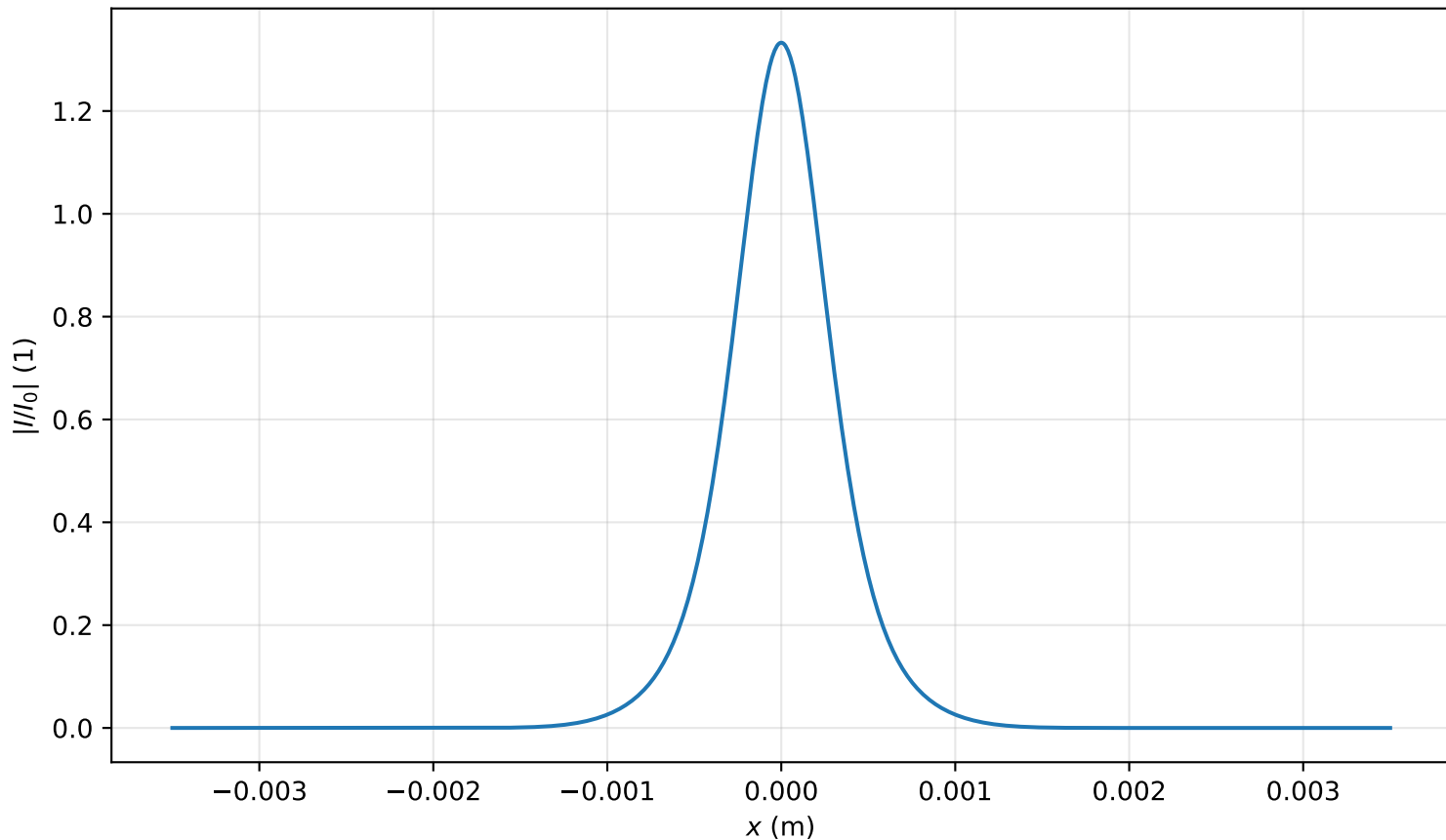
Intensity profile I(x, y = 0, z = 1.194m)/I_0 , P_{in}=0.8P_{cr} , artificial time
